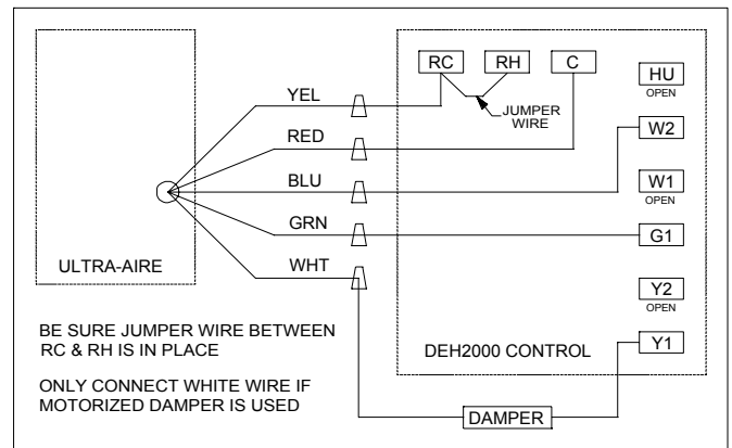
Wiring Diagram
